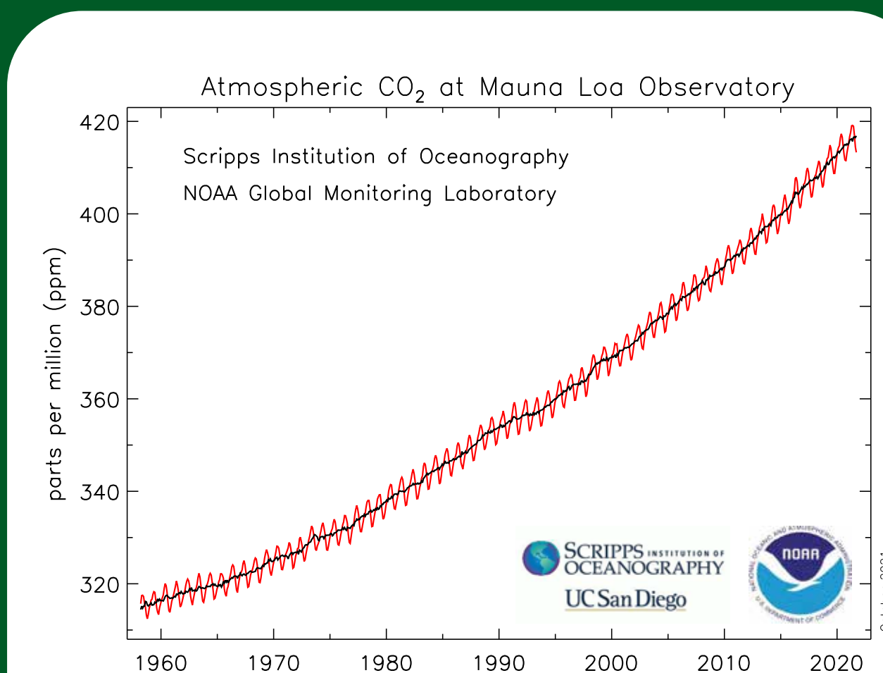
Figure 2: Increase of carbon dioxide concentration in the atmosphere in the period 1960-2020
